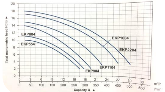
HYDRAULIC PERFORMANCE CURVE
