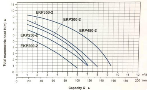
HYDRAULIC PERFORMANCE CURVE
